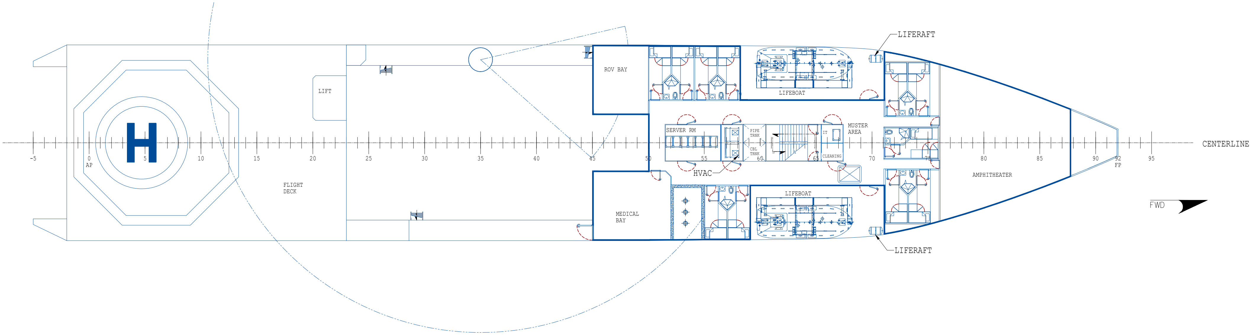
PLAN 3-C5 LVL 4, FOCSLE DECK LOOKING DOWN
