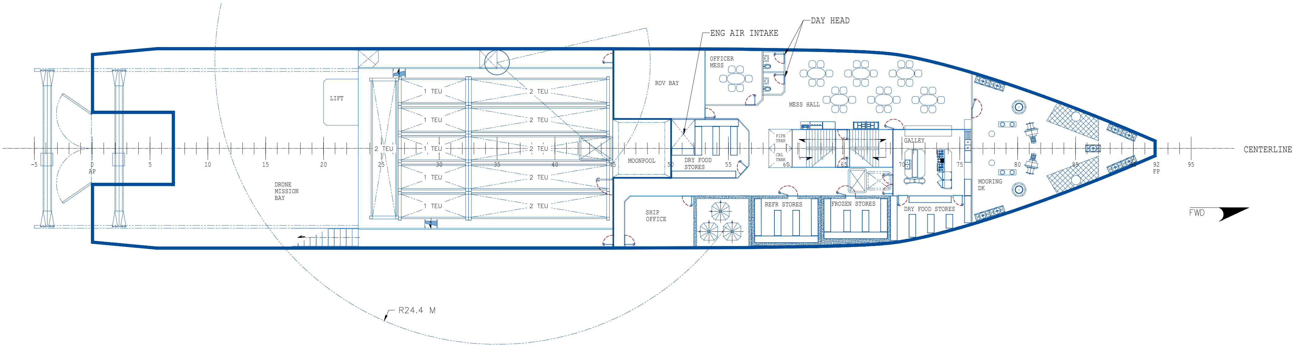
PLAN 3-A5 LVL 3, MAIN DECK LOOKING DOWN
